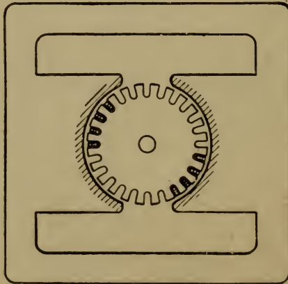
Figure 30 Iron clad armature.
